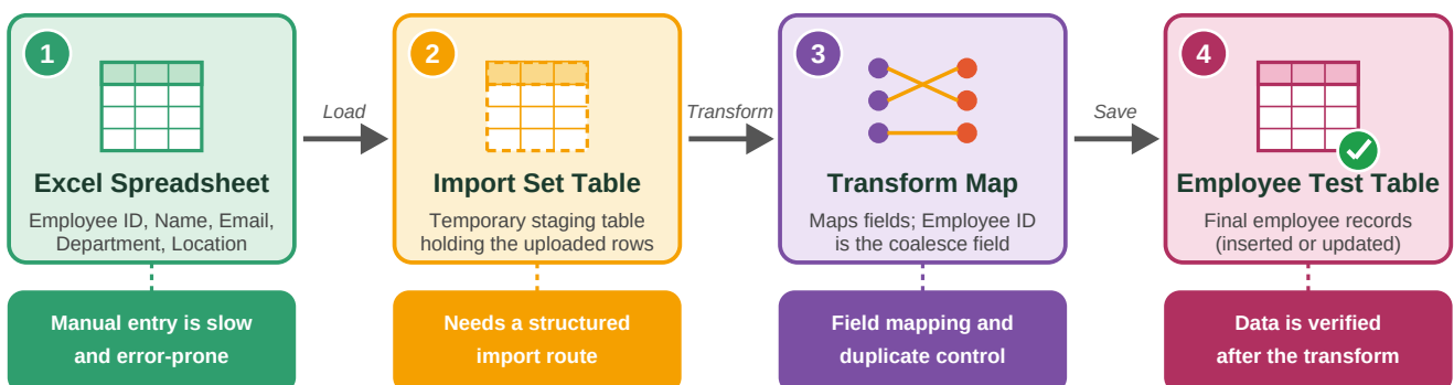
Figure: Spreadsheet data flows through a staging table and a Transform Map into the Employee Test table. The coloured boxes show the user need each stage addresses.
